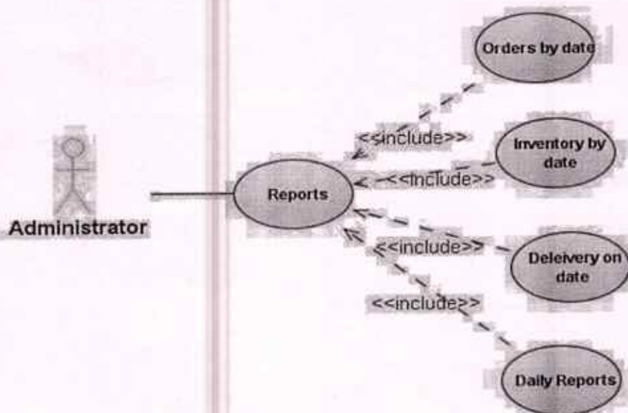
Fig: 2.4.4. Use case diagram for reports.
