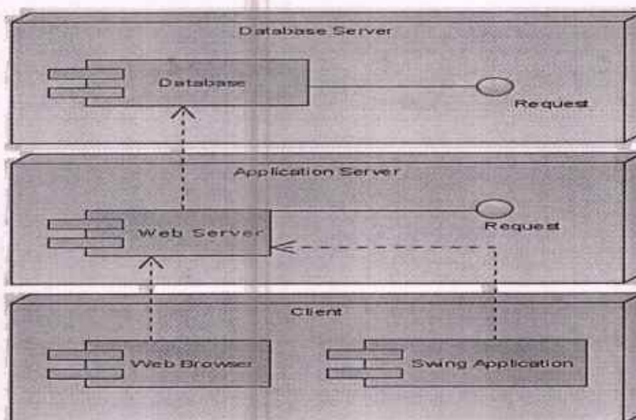
Fig: 2.4.8. Deployment diagram one.
