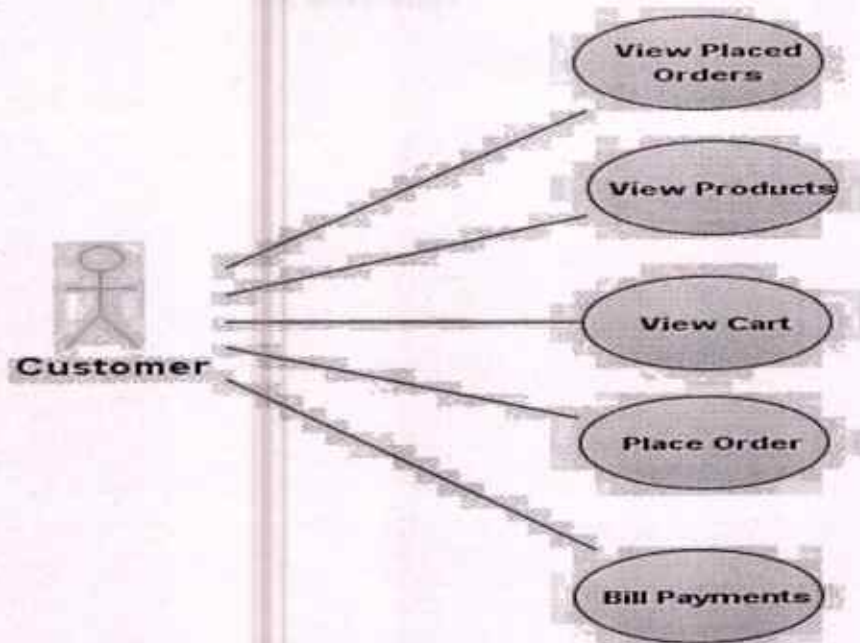
Fig: 2.4.2. Use case diagram for Customer.
